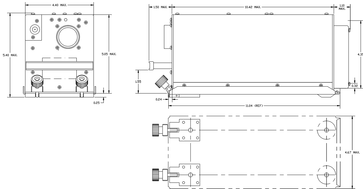
Figure 31. Flexcomm RT-406F Outline Drawing Portions of Dwg No. 147-0119-000
