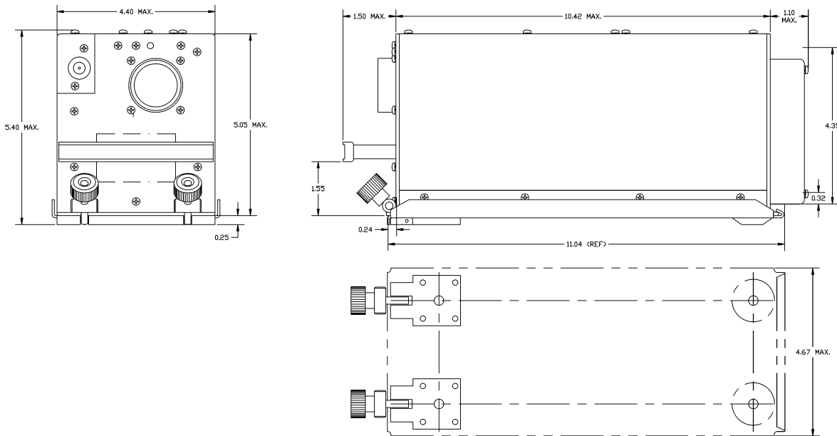
Figure 30. Flexcomm RT-138F Outline Drawing Portions of Dwg No. 147-0119-000
